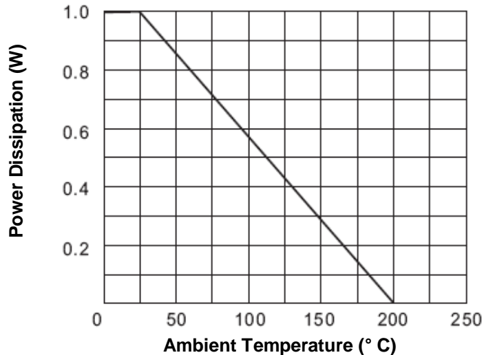
Fig.1-Power Derating Curve
