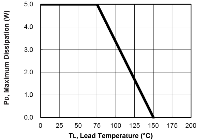
Fig.1- Power Temperature Derating Curve
