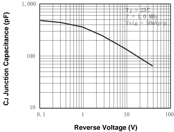
Fig.5- Typical Junction Capacitance Per Bridge Element
