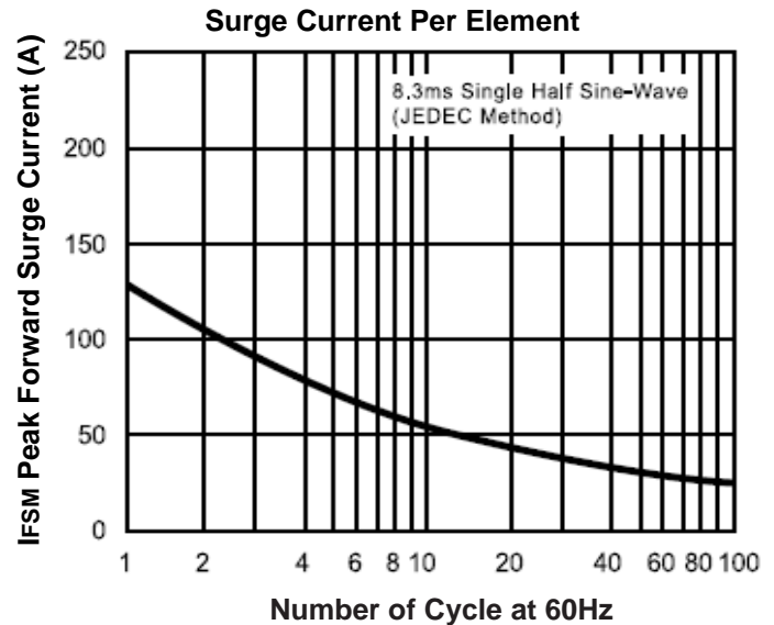
Fig.2- Maximum Non-Repetitive Peak Forward Surge Current Per Element
