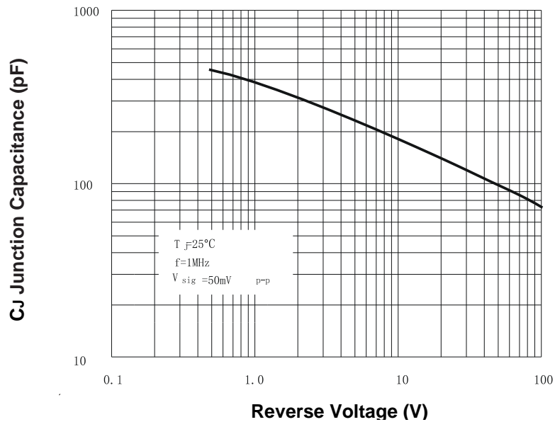
Fig.5-Typical junction capacitance
