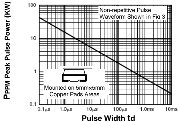
Fig.2- Peak Pulse Power Rating Curve
