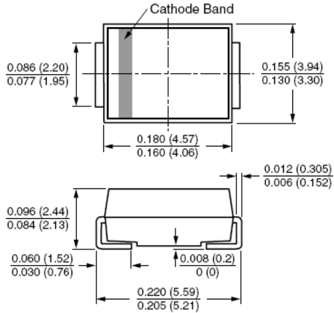
DO-214AA (SMB)
