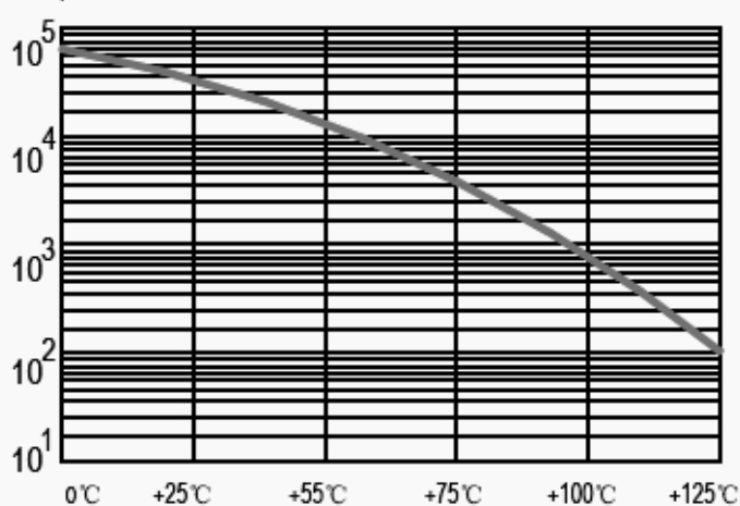
MΩμF Time constant VS. temperature
