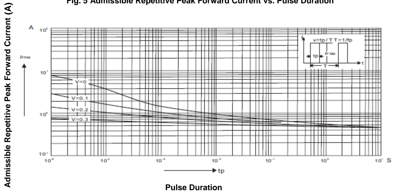
Fig. 5 Admissible Repetitive Peak Forward Current vs. Pulse Duration
