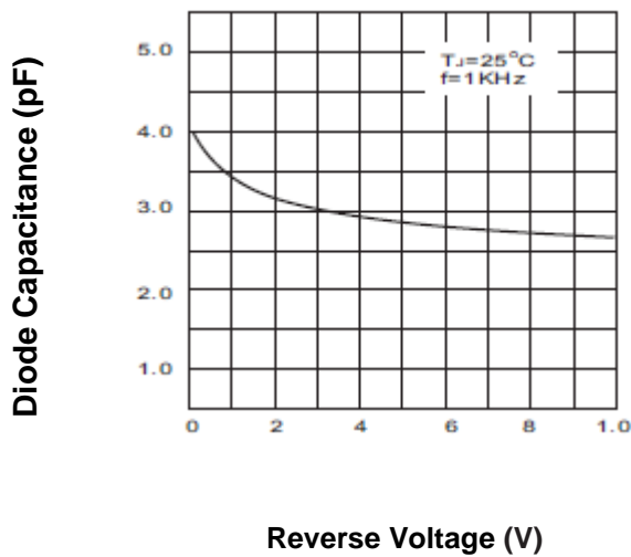
Fig.3- Junction Capacitance Curve
