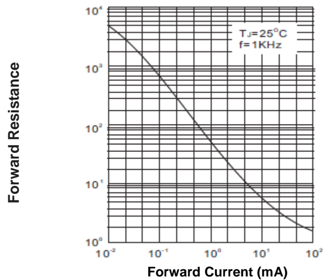
Fig.4- Forward Resistance vs. Forward Current
