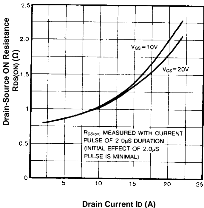
Fig.12- Typical On-Resistance Vs. Drain Current
