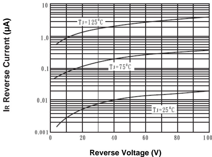
Fig.3- Typical Instantaneous Reverse Characteristics
