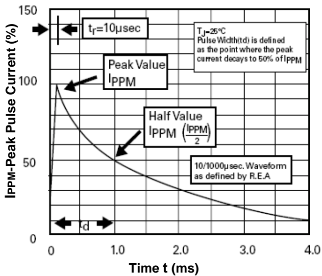
Fig.3- Pulse Waveform
